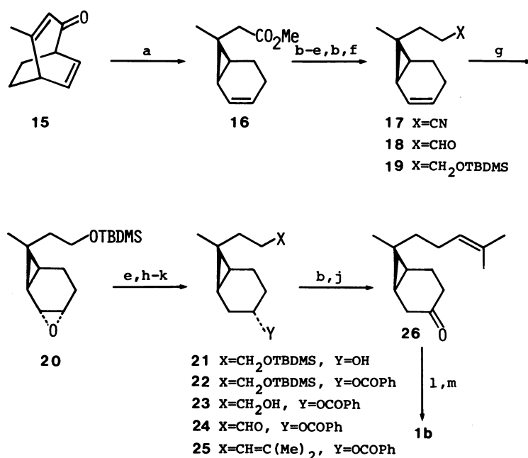
Scheme 3. Synthesis of (±)-isosquicarenene. a)
